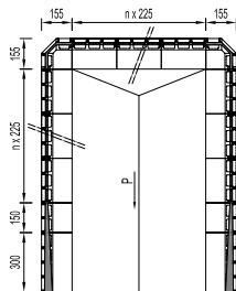
ENOSTAVEN SILOS
