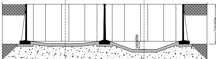
EXAMPLE OF LAYOUT OF BUNKER SILO OVER THE GROUND – PARTIALLY ON THE GROUND – ON THE GROUND
