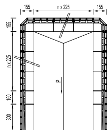
ENOSTAVEN SILOS
