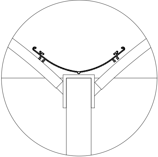
DETAIL "A": Galvanized "U"-shaped plate for fixing the structure to the precast reinforced concrete wall.
